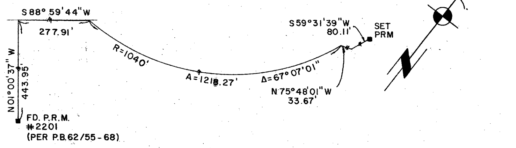
DETAIL (NOT TO SCALE)
